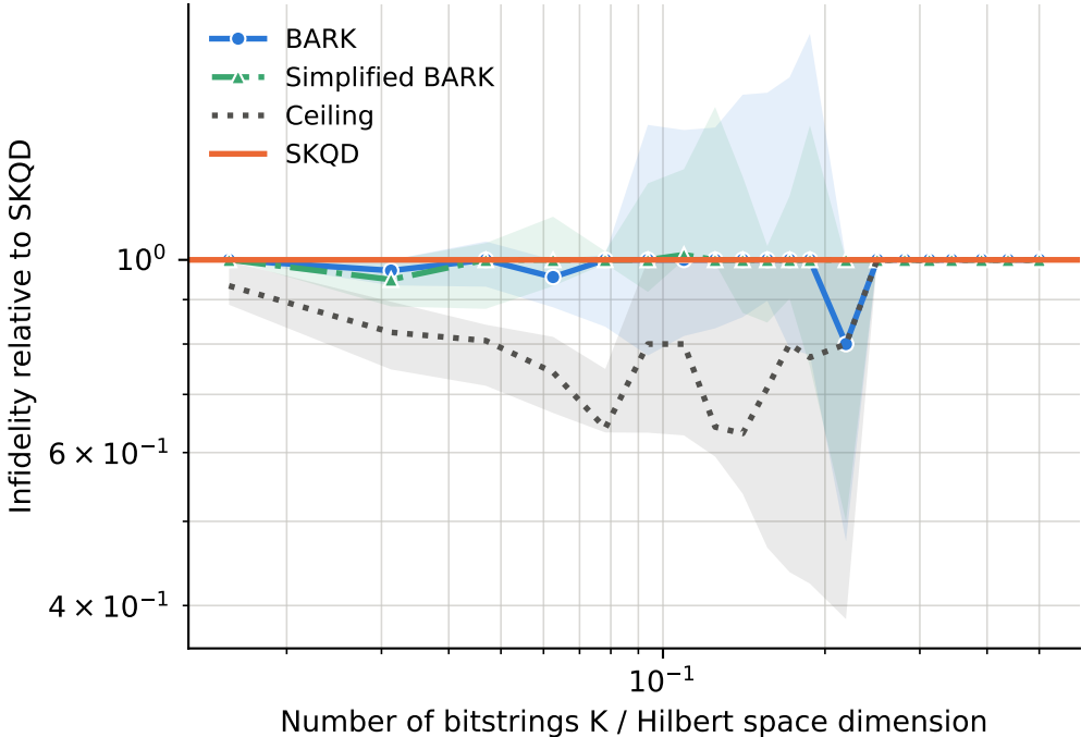
runs per point -- BARK: 25, Ceiling: 25, SKQD: 25, Simplified BARK: 25
