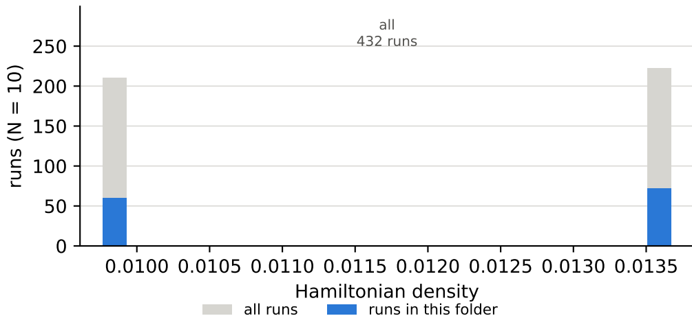
Hamiltonian density over all runs, and the cuts behind the bins N = 10, anisotropy delta = 0.5
