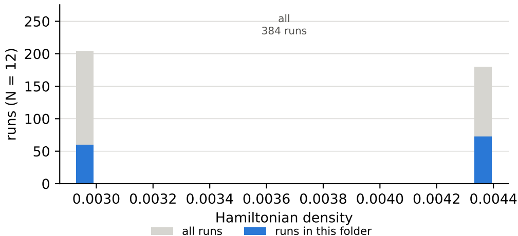
Hamiltonian density over all runs, and the cuts behind the bins N = 12 , anisotropy \delta = 0.5
