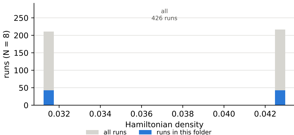
Hamiltonian density over all runs, and the cuts behind the bins N = 8 , anisotropy \delta = 10
