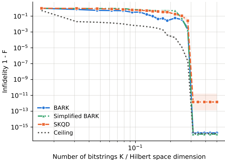
N = 6, anisotropy delta = 10, field B_z = high (band: standard error)
