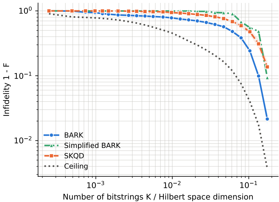
runs per point -- BARK: 12, Ceiling: 12, SKQD: 12, Simplified BARK: 12
