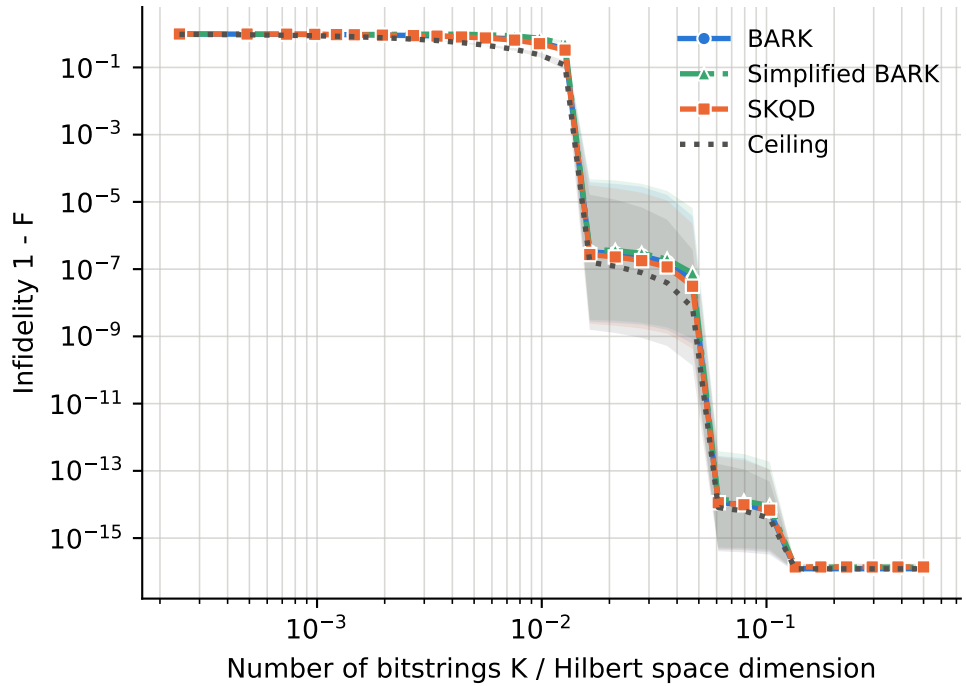
runs per point -- BARK: 15, Ceiling: 15, SKQD: 15, Simplified BARK: 15
