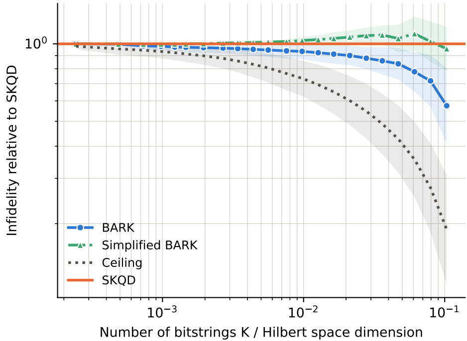
runs per point -- BARK: 27, Ceiling: 27, SKQD: 27, Simplified BARK: 27
