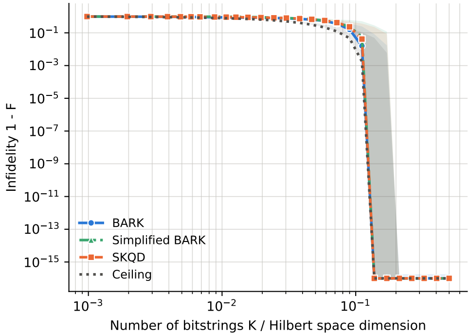
runs per point -- BARK: 14, Ceiling: 14, SKQD: 14, Simplified BARK: 14
