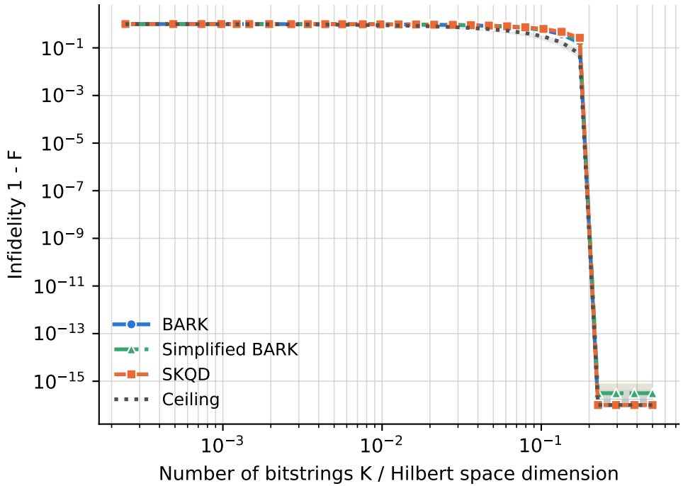
runs per point -- BARK: 24, Ceiling: 24, SKQD: 24, Simplified BARK: 24
