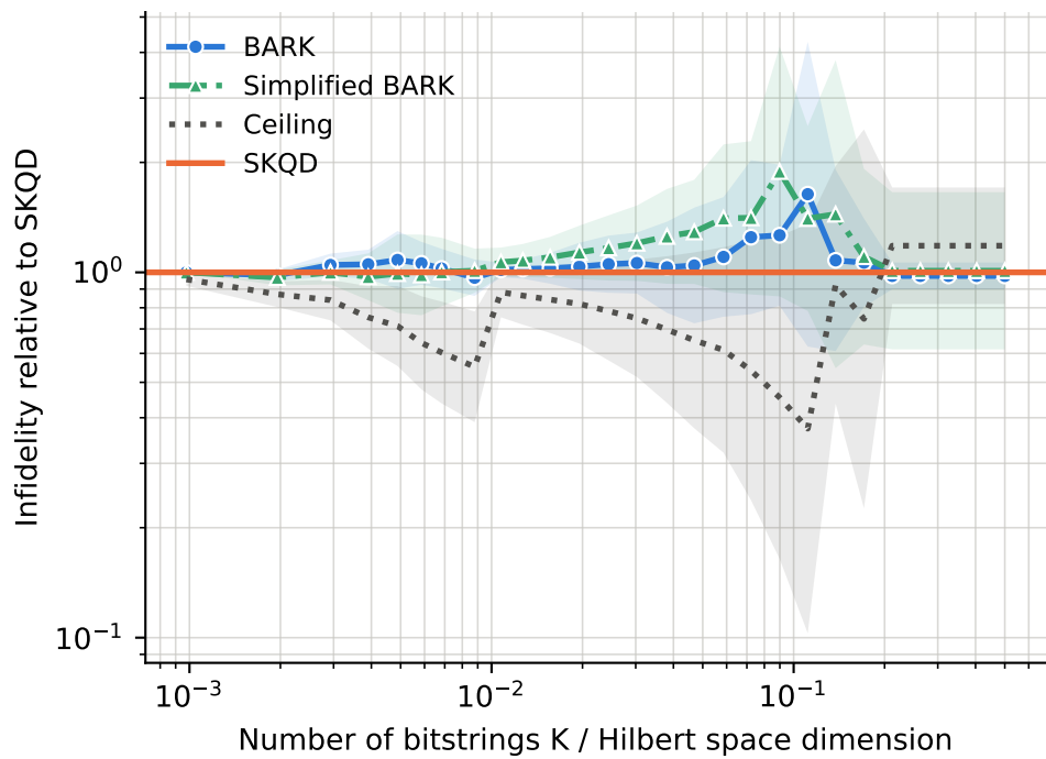
runs per point -- BARK: 11, Ceiling: 11, SKQD: 11, Simplified BARK: 11
