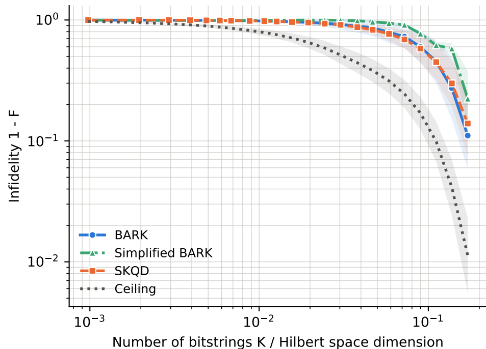
runs per point -- BARK: 20, Ceiling: 20, SKQD: 20, Simplified BARK: 20
