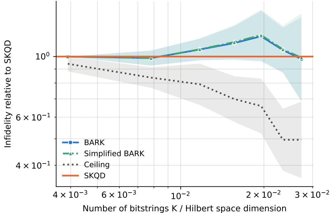
runs per point -- BARK: 8, Ceiling: 8, SKQD: 8, Simplified BARK: 8
