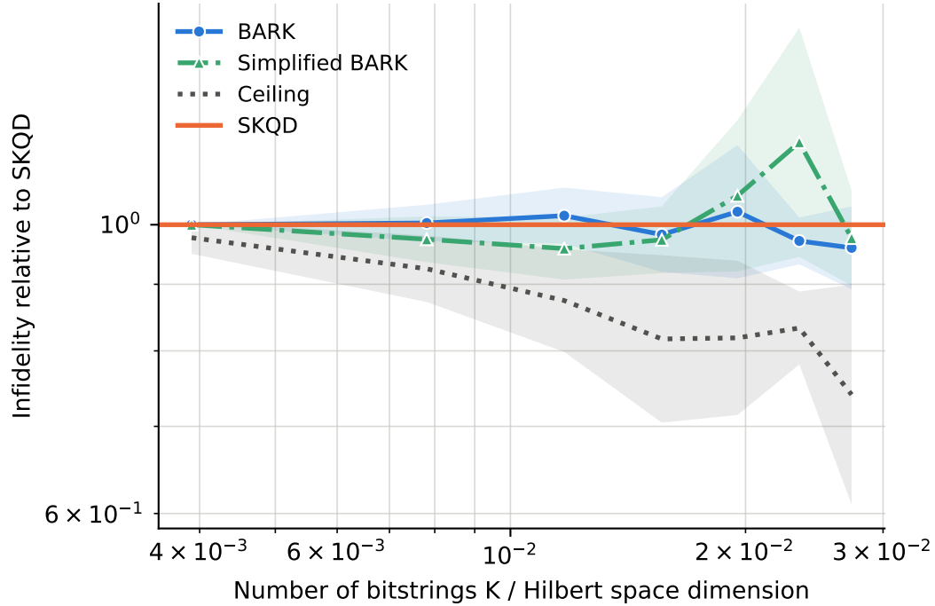
runs per point -- BARK: 13, Ceiling: 13, SKQD: 13, Simplified BARK: 13
