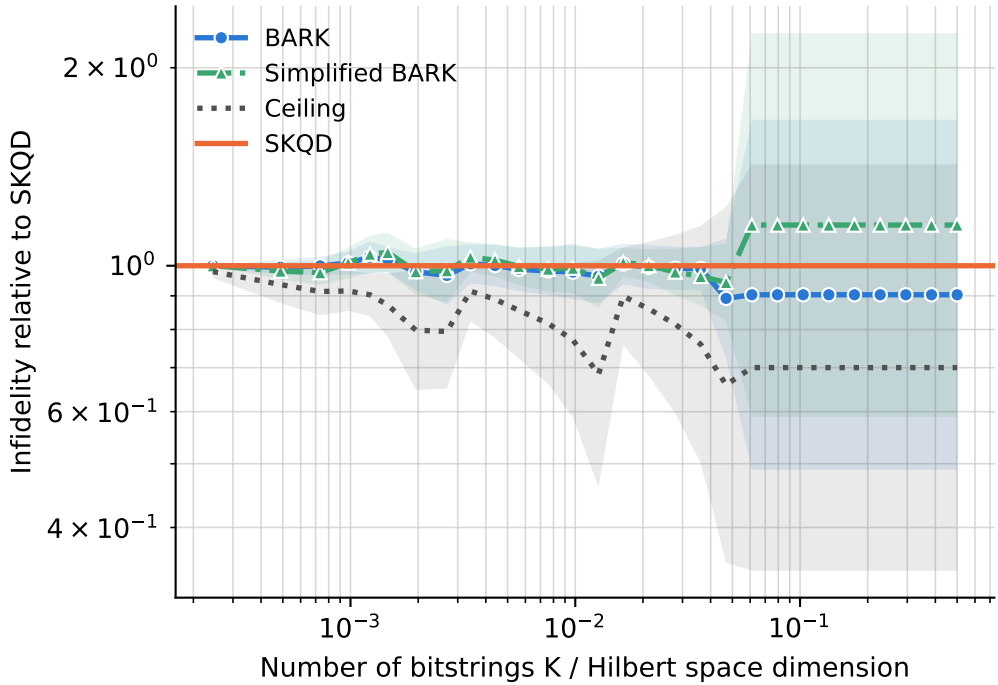
runs per point -- BARK: 18, Ceiling: 18, SKQD: 18, Simplified BARK: 18
