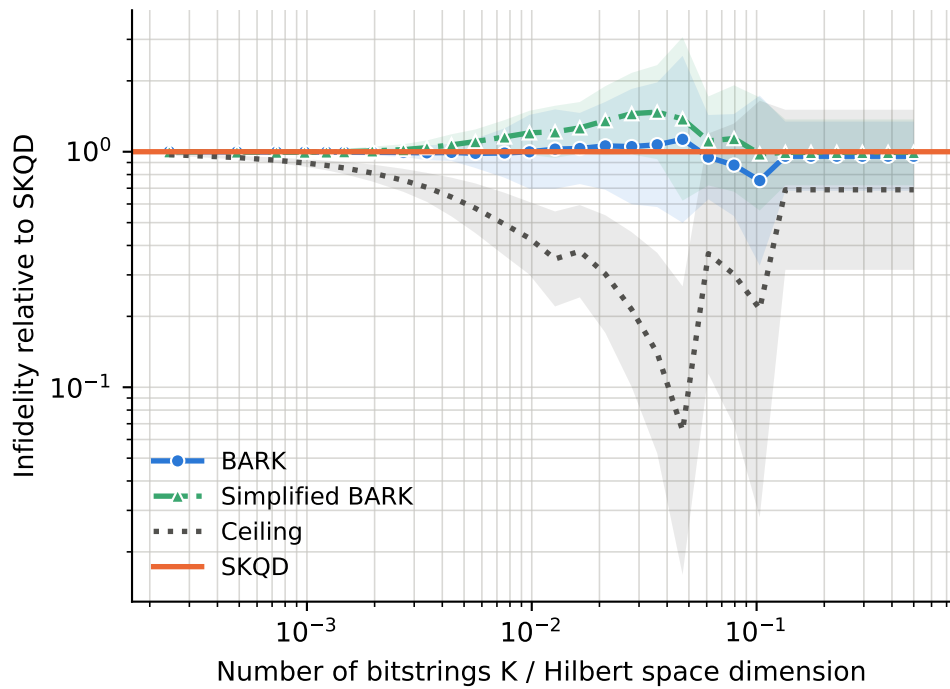
runs per point -- BARK: 48, Ceiling: 48, SKQD: 48, Simplified BARK: 48
