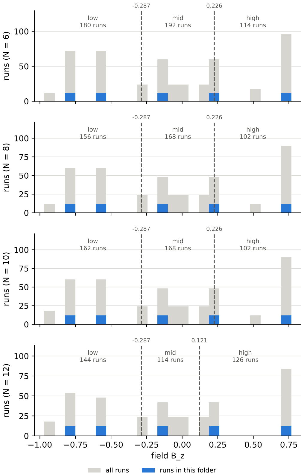
field B z over all runs, and the cuts behind the bins anisotropy \delta = 1
