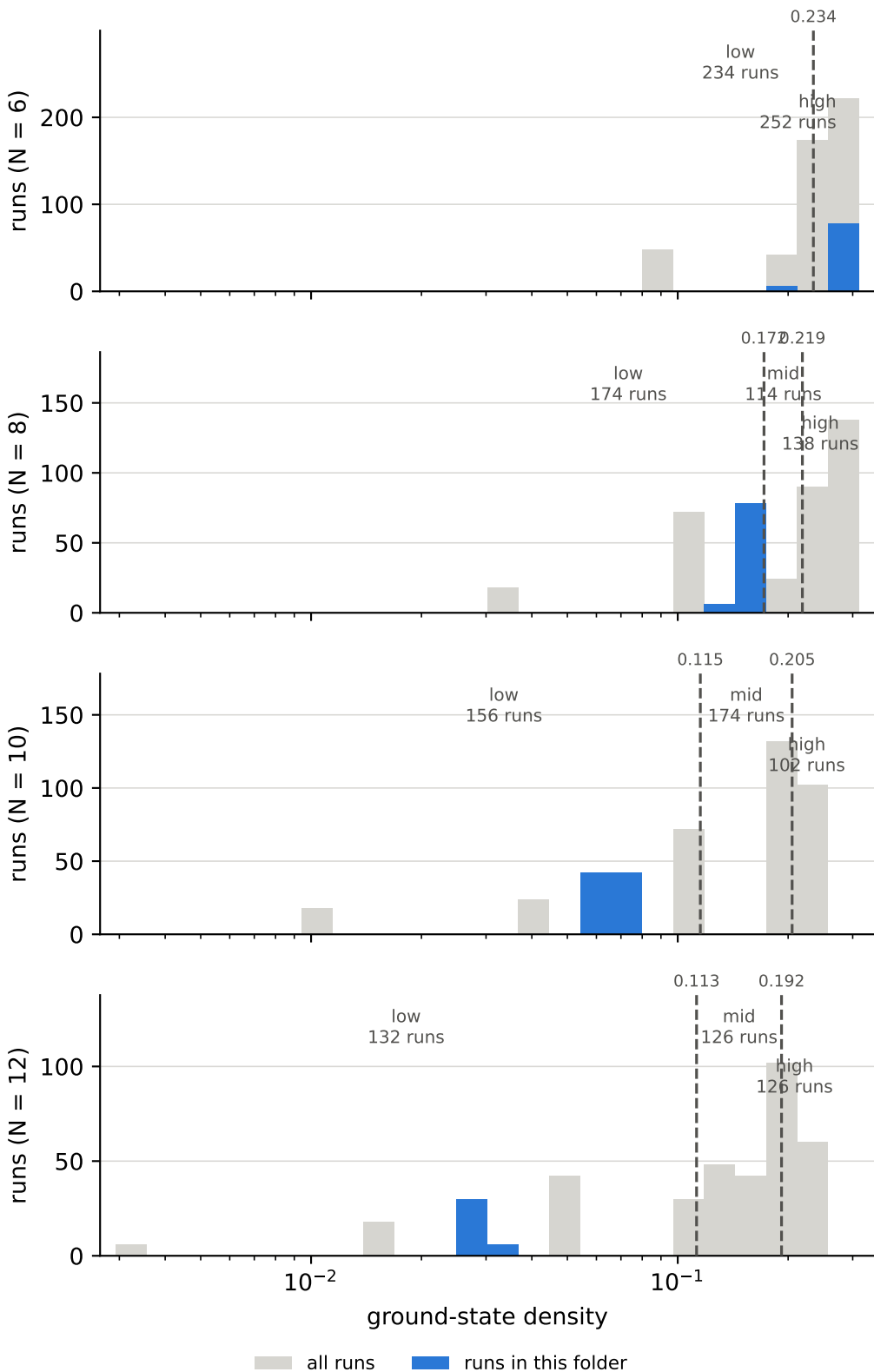
ground-state density over all runs, and the cuts behind the bins anisotropy \Delta = 10
