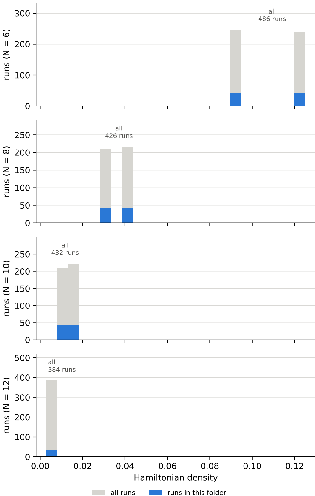
Hamiltonian density over all runs, and the cuts behind the bins anisotropy delta = 10
