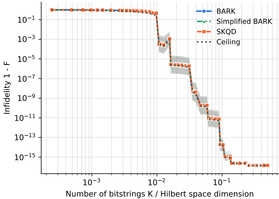
runs per point -- BARK: 19-70, Ceiling: 19-70, SKQD: 19-70, Simplified BARK: 19-70
