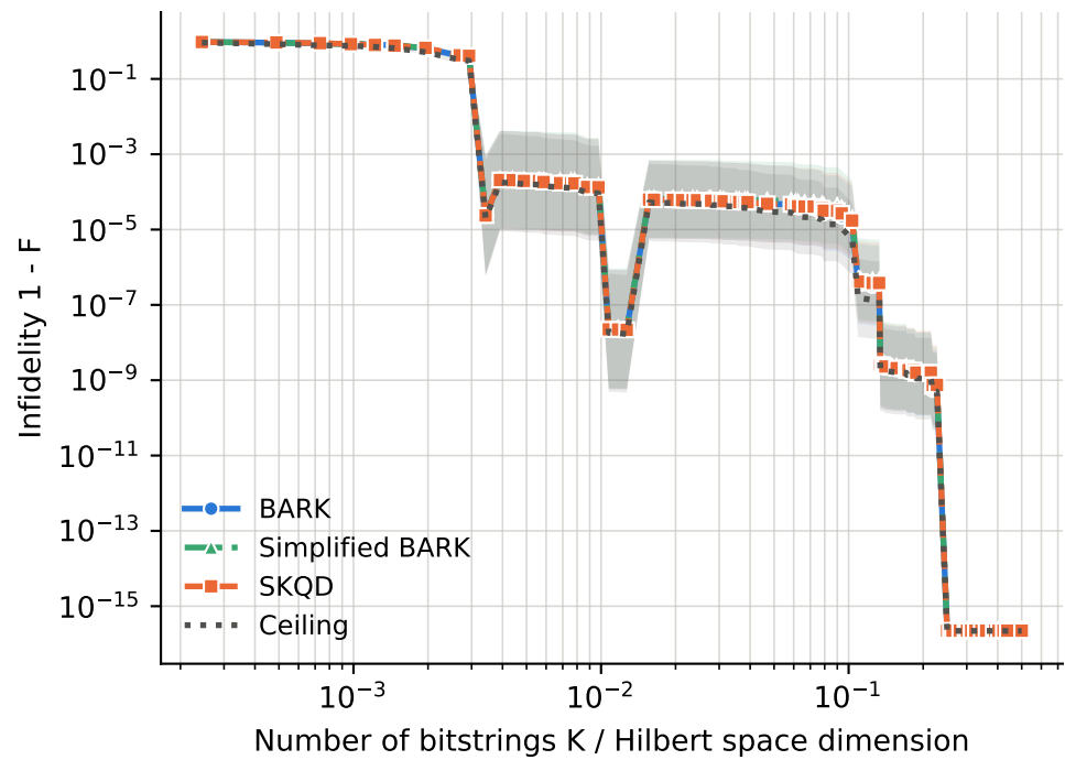
runs per point -- BARK: 13-44, Ceiling: 13-44, SKQD: 13-44, Simplified BARK: 13-44
