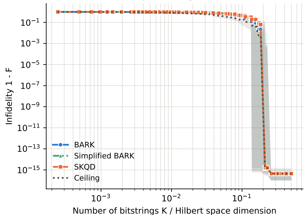
runs per point -- BARK: 5-24, Ceiling: 5-24, SKQD: 5-24, Simplified BARK: 5-24
