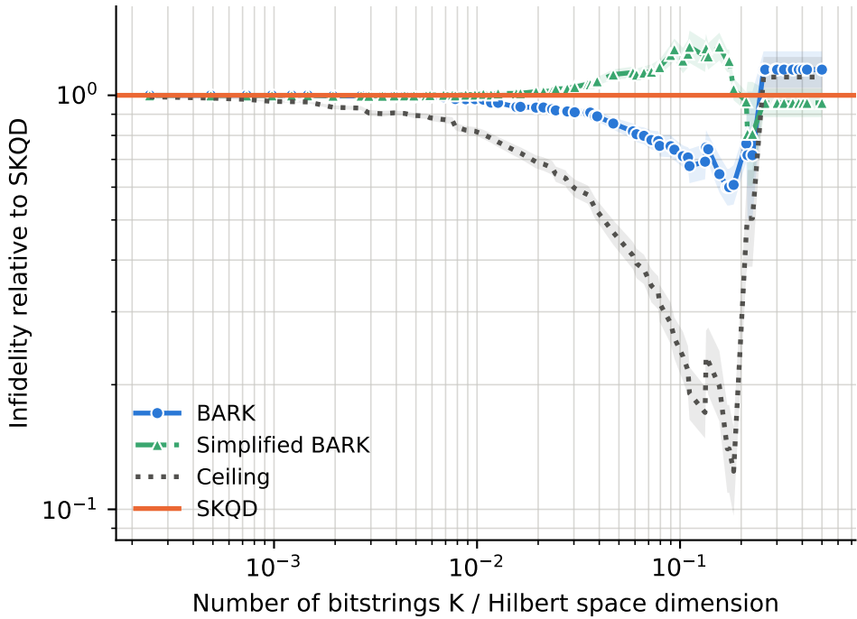
runs per point -- BARK: 5-38, Ceiling: 5-38, SKQD: 5-38, Simplified BARK: 5-38
