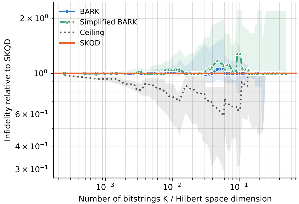
runs per point -- BARK: 8-48, Ceiling: 8-48, SKQD: 8-48, Simplified BARK: 8-48
