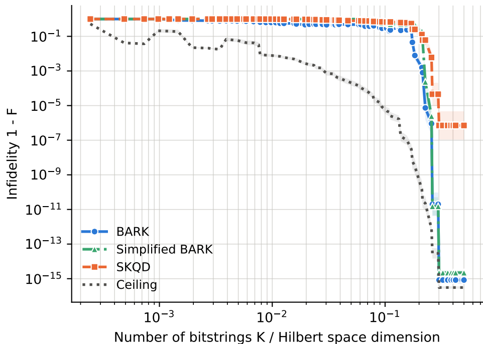
runs per point -- BARK: 11-58, Ceiling: 11-58, SKQD: 11-58, Simplified BARK: 11-58
