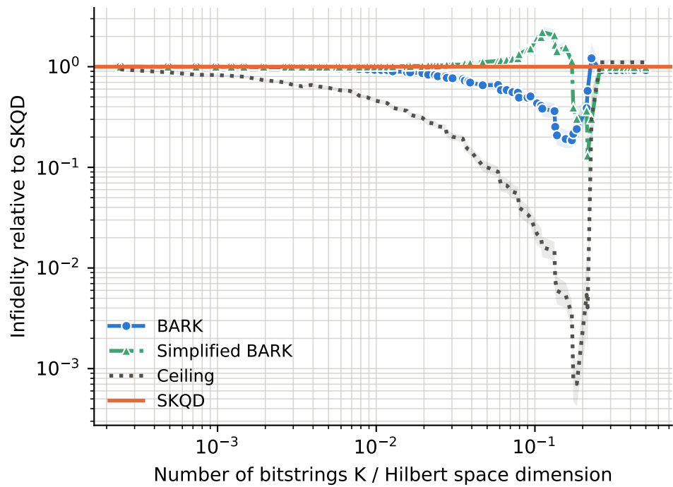
runs per point -- BARK: 12-25, Ceiling: 12-25, SKQD: 12-25, Simplified BARK: 12-25
