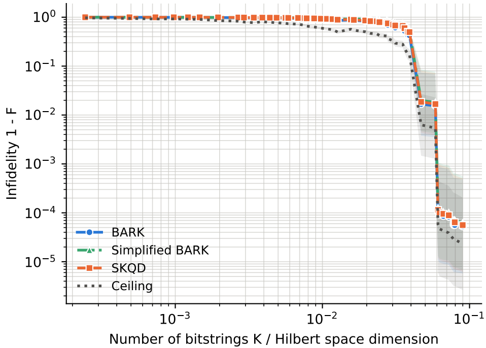
runs per point -- BARK: 7-45, Ceiling: 7-45, SKQD: 7-45, Simplified BARK: 7-45
