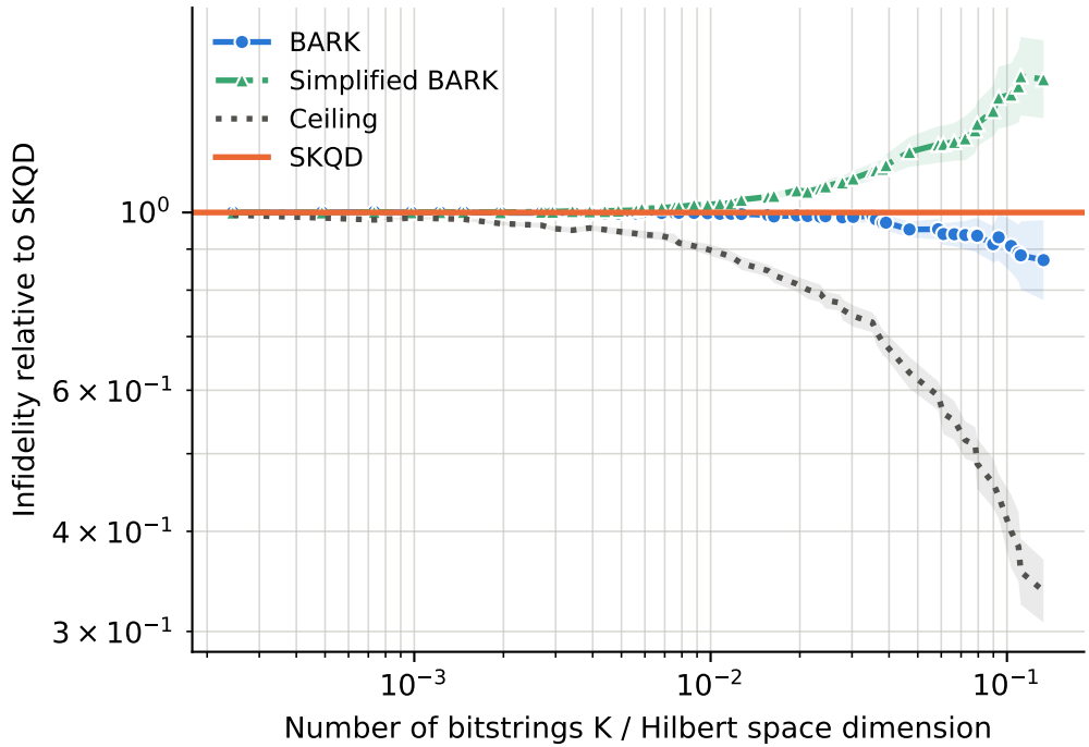
runs per point -- BARK: 4-18, Ceiling: 4-18, SKQD: 4-18, Simplified BARK: 4-18
