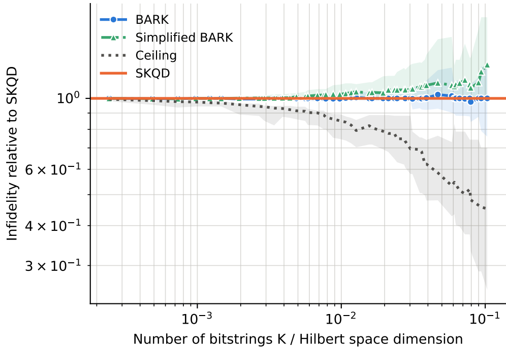
runs per point -- BARK: 18-74, Ceiling: 18-74, SKQD: 18-74, Simplified BARK: 18-74
