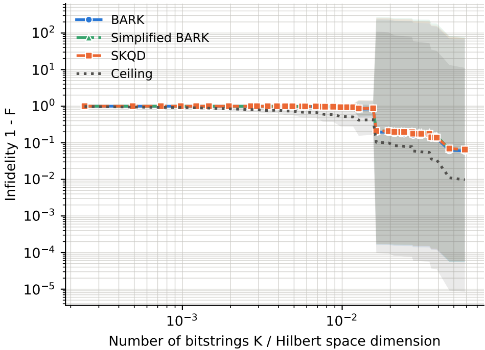
runs per point -- BARK: 12-22, Ceiling: 12-22, SKQD: 12-22, Simplified BARK: 12-22
