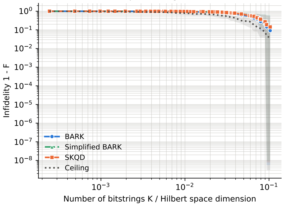
runs per point -- BARK: 15-75, Ceiling: 15-75, SKQD: 15-75, Simplified BARK: 15-75
