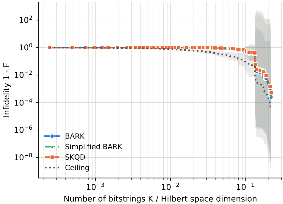
runs per point -- BARK: 18-38, Ceiling: 18-38, SKQD: 18-38, Simplified BARK: 18-38
