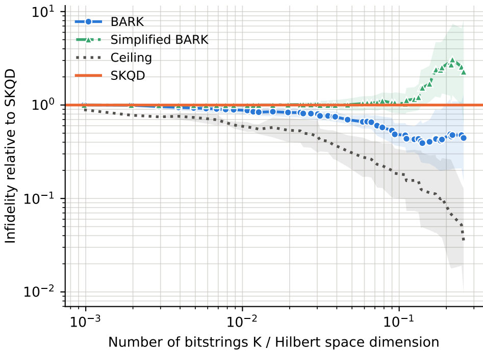
runs per point -- BARK: 12-24, Ceiling: 12-24, SKQD: 12-24, Simplified BARK: 12-24
