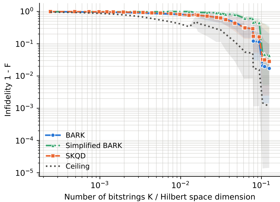
runs per point -- BARK: 7-12, Ceiling: 7-12, SKQD: 7-12, Simplified BARK: 7-12
