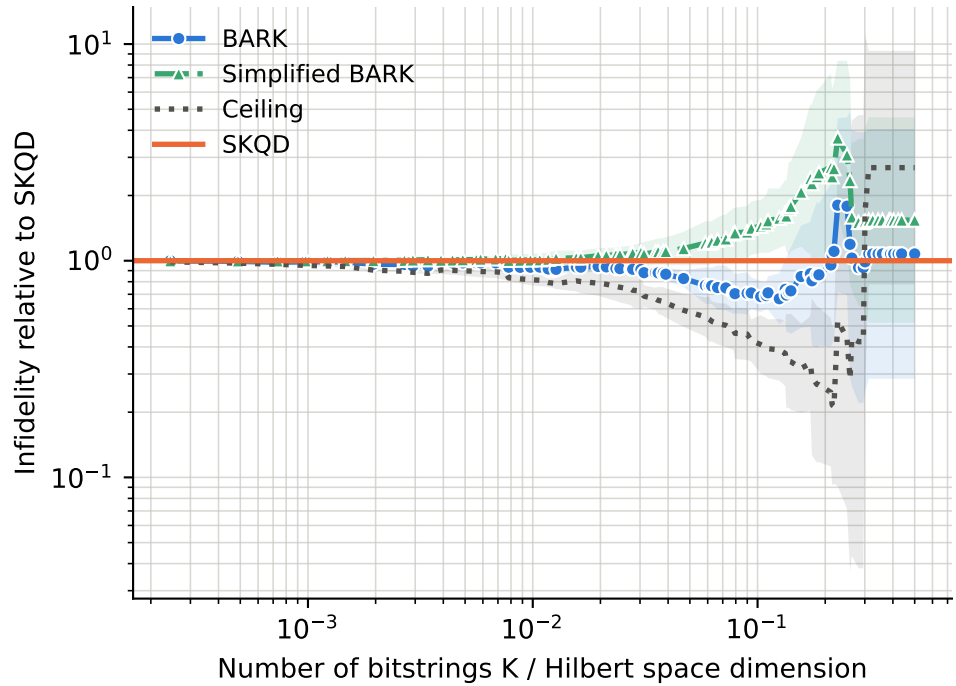
runs per point -- BARK: 2-14, Ceiling: 2-14, SKQD: 2-14, Simplified BARK: 2-14
