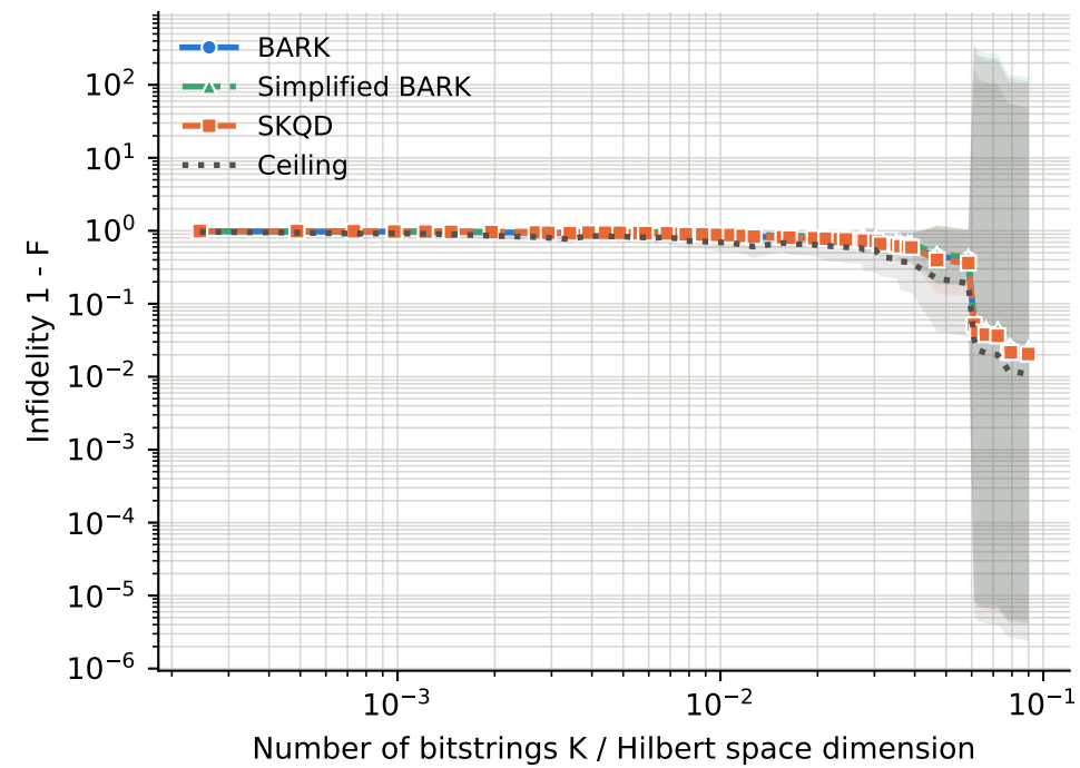
runs per point -- BARK: 2-33, Ceiling: 2-33, SKQD: 2-33, Simplified BARK: 2-33
