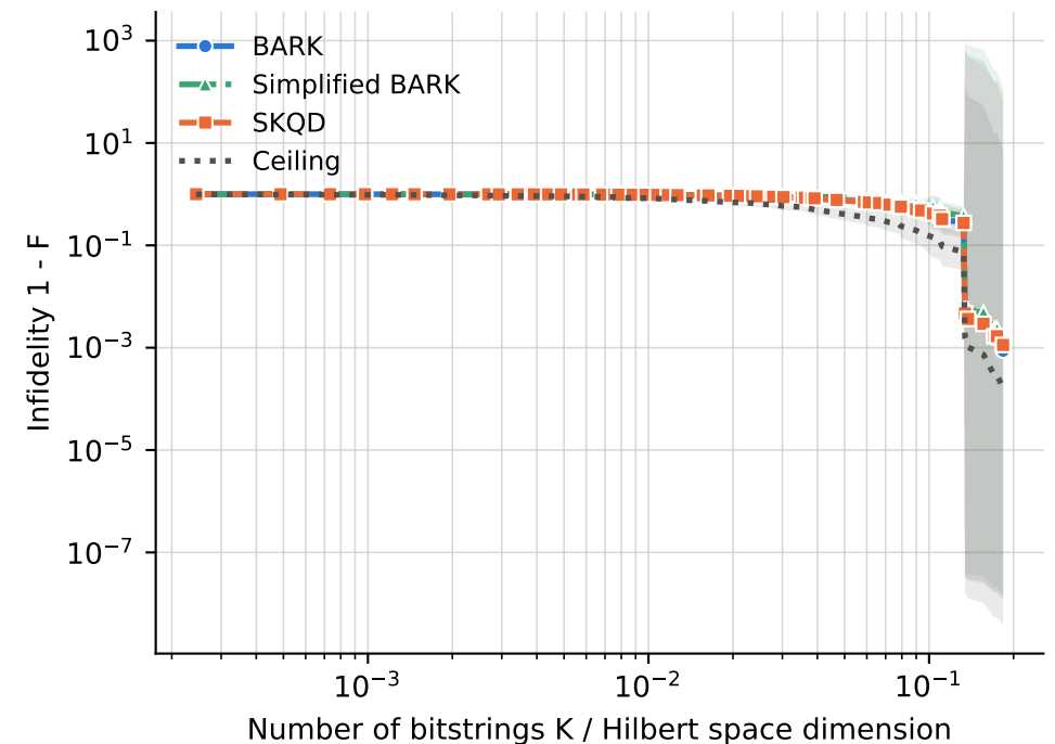
runs per point -- BARK: 2-17, Ceiling: 2-17, SKQD: 2-17, Simplified BARK: 2-17
