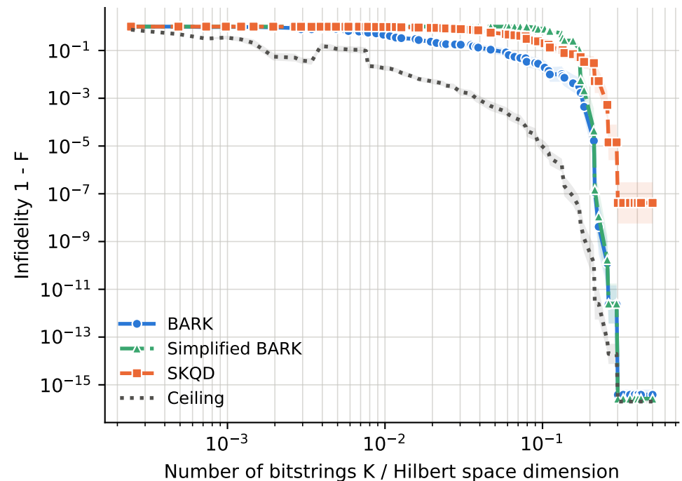
runs per point -- BARK: 6-37, Ceiling: 6-37, SKQD: 6-37, Simplified BARK: 6-37
