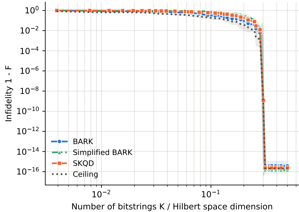
runs per point -- BARK: 4-8, Ceiling: 4-8, SKQD: 4-8, Simplified BARK: 4-8
