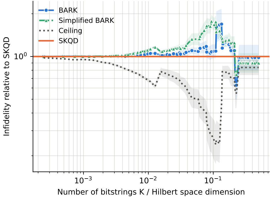
runs per point -- BARK: 3-17, Ceiling: 3-17, SKQD: 3-17, Simplified BARK: 3-17
