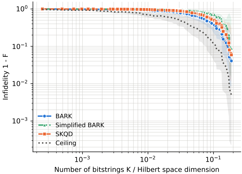
runs per point -- BARK: 12-84, Ceiling: 12-84, SKQD: 12-84, Simplified BARK: 12-84
