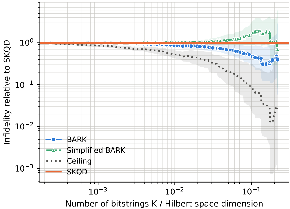
runs per point -- BARK: 24-72, Ceiling: 24-72, SKQD: 24-72, Simplified BARK: 24-72
