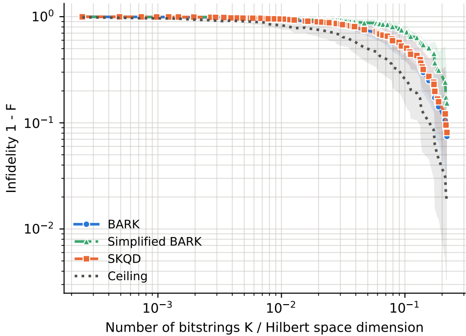
runs per point -- BARK: 7-40, Ceiling: 7-40, SKQD: 7-40, Simplified BARK: 7-40
