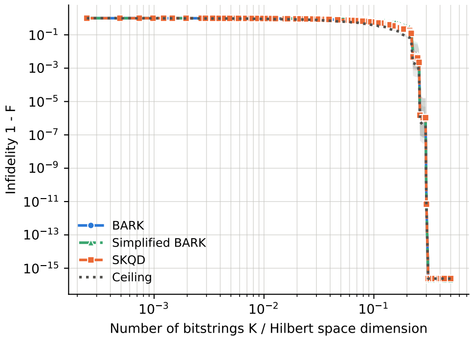
runs per point -- BARK: 3-32, Ceiling: 3-32, SKQD: 3-32, Simplified BARK: 3-32
