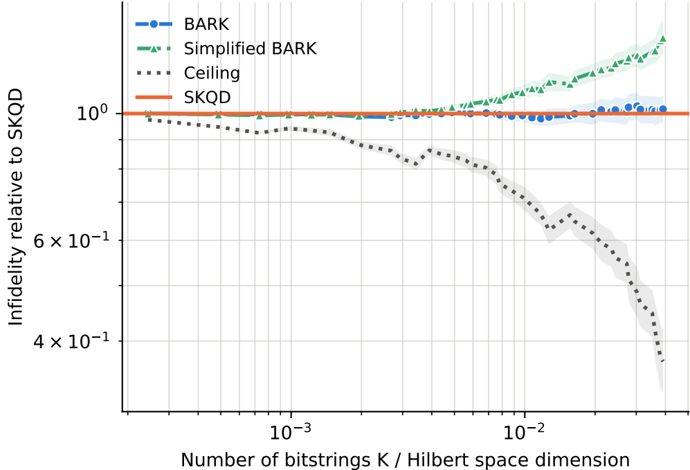
runs per point -- BARK: 7-51, Ceiling: 7-51, SKQD: 7-51, Simplified BARK: 7-51
