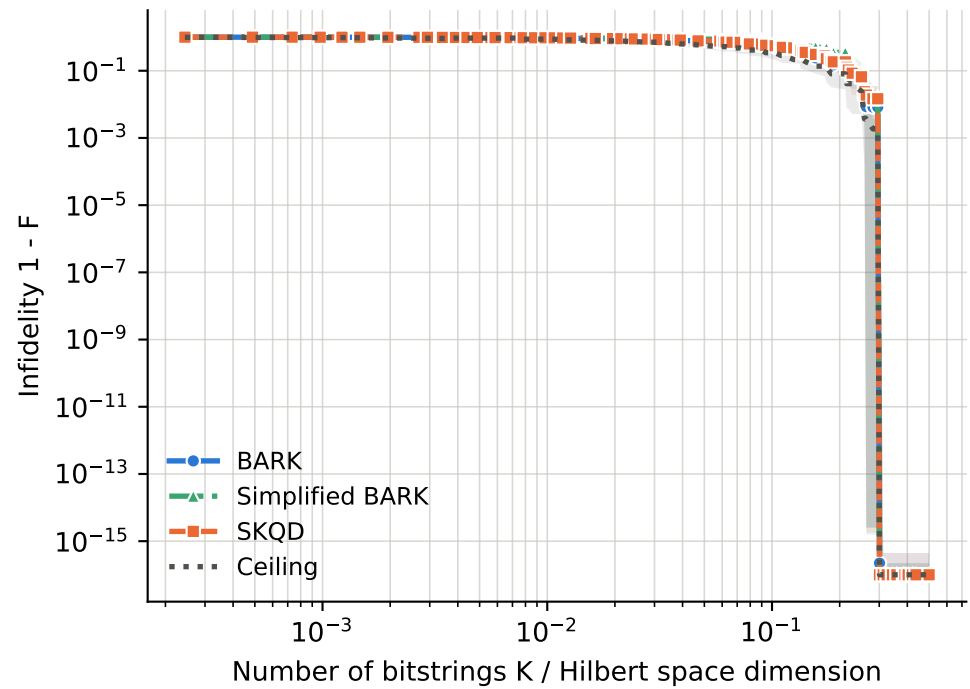
runs per point -- BARK: 8-47, Ceiling: 8-47, SKQD: 8-47, Simplified BARK: 8-47
