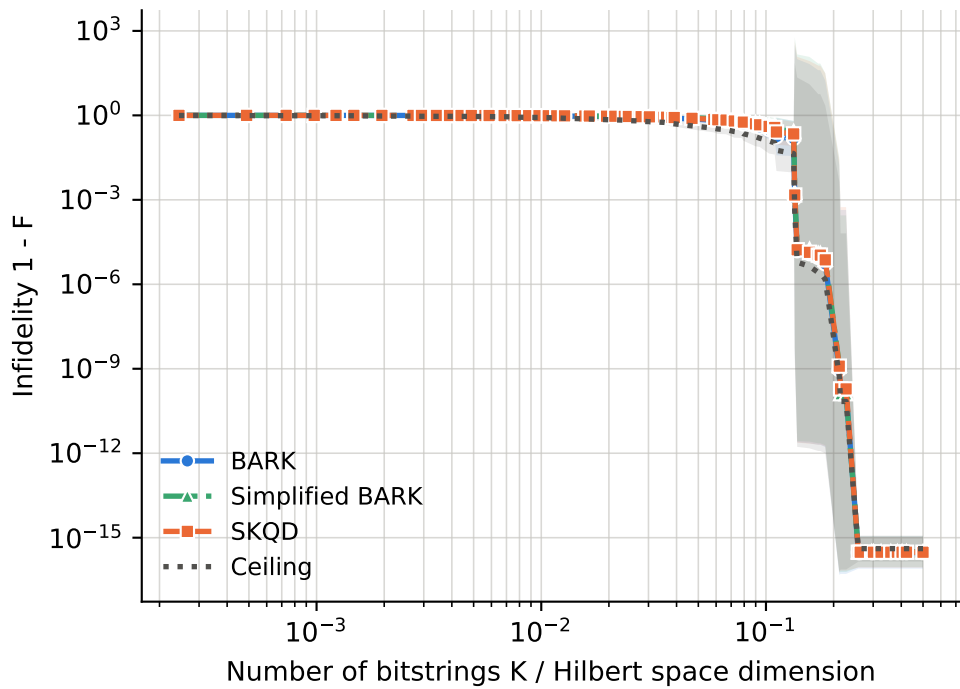
runs per point -- BARK: 5-35, Ceiling: 5-35, SKQD: 5-35, Simplified BARK: 5-35
