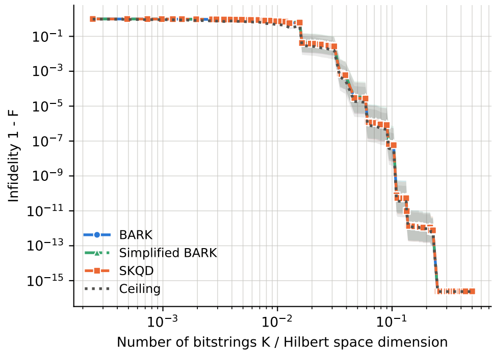
runs per point -- BARK: 13-57, Ceiling: 13-57, SKQD: 13-57, Simplified BARK: 13-57
