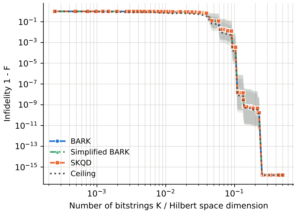
runs per point -- BARK: 2-21, Ceiling: 2-21, SKQD: 2-21, Simplified BARK: 2-21
