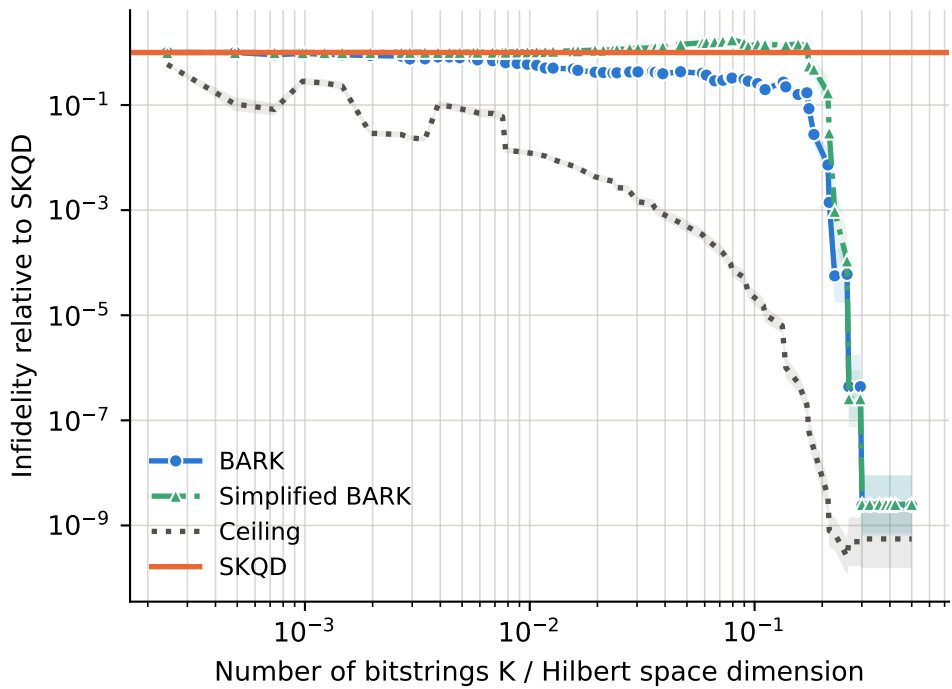
runs per point -- BARK: 16-113, Ceiling: 16-113, SKQD: 16-113, Simplified BARK: 16-113
